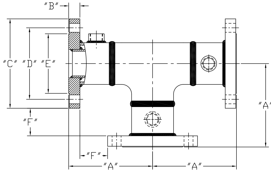
DIMENSIONS (ALL ARE IN INCHES)
