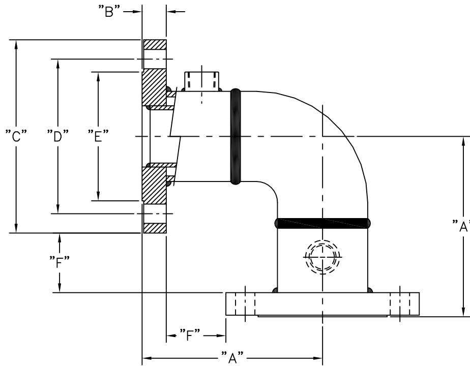
DIMENSIONS (ALL ARE IN INCHES)
